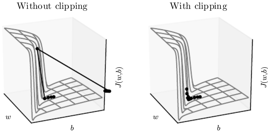
Figure 10.18: Example of the effect of gradient clipping in a recurrent network with two parameters w and b . Gradient clipping can make gradient descent perform more reasonably in the vicinity of extremely steep cliffs. These steep cliffs commonly occur in recurrent networks near where a recurrent network behaves approximately linearly. The cliff is exponentially steep in the number of time steps because the weight matrix is multiplied by itself once for each time step. ( Left ) Gradient descent without gradient clipping overshoots the bottom of this small ravine, then receives a very large gradient from the cliff face. The large gradient catastrophically propels the parameters outside the axes of the plot. ( Right ) Gradient descent with gradient clipping has a more moderate reaction to the cliff. While it does ascend the cliff face, the step size is restricted so that it cannot be propelled away from steep region near the solution. Figure adapted with permission from Pascanu et al. (2013a).
